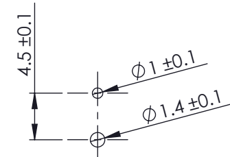
RECOMMENDED PCB HOLE LAYOUT
