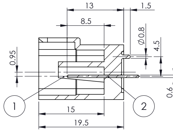
SECTION X-X
