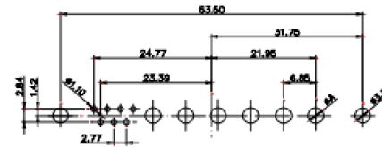
13W6 Female
