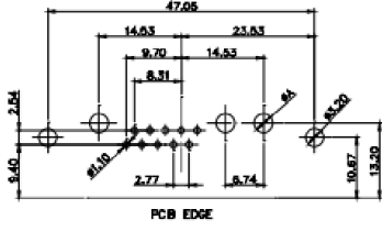
13W6 Female
