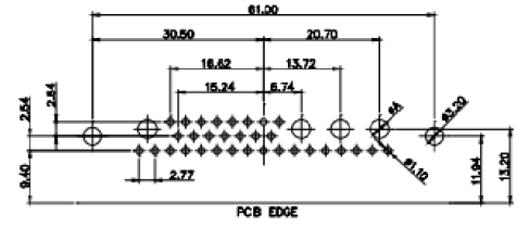
43W2 Female
