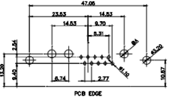
13W6 Male
