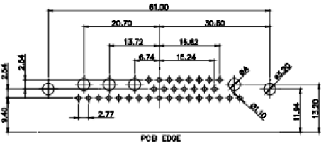
43W2 Male
