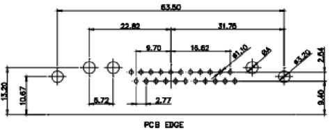
36W4 Male
