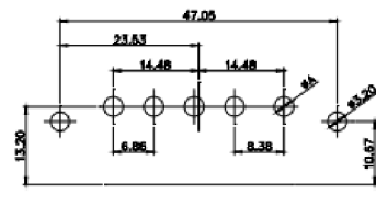
5W5 Female
