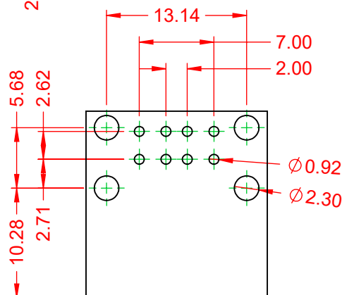
RECOMMENDED P.C.B HOLE LAYOUT TOP VIEW (TOLERANCE:±0.10)
