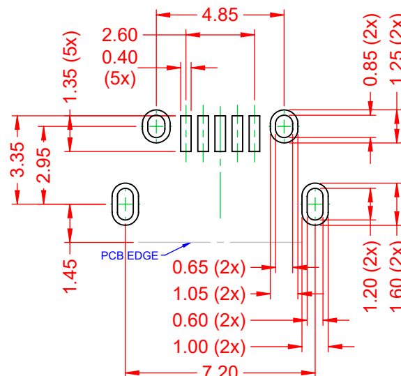
RECOMMENDED P.C.B HOLE LAYOUT TOP VIEW - TOL' = ±0.05
