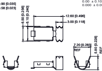
TOP METAL SHELL
