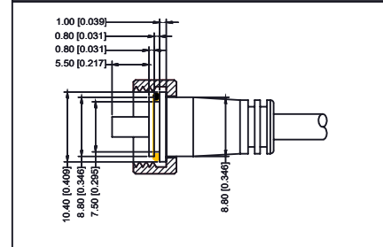
RECOMMENDED ASSEMBLY
