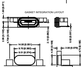
PANEL MOUNTING LAYOUT
